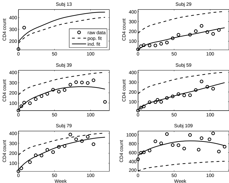
Figure 17.9 Type 1 SPME Modeling of the ACTG 388 Data: Raw Data (circles), Population Fits (dashed curves) and Individual Fits (solid curves) for Six Selected Subjects
